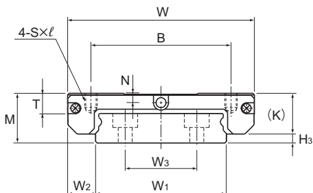
Models SRS15WM/WN
