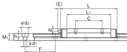
Models RSR15WV/WVM/WWN
